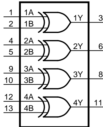
Figure 1. Logic symbol
